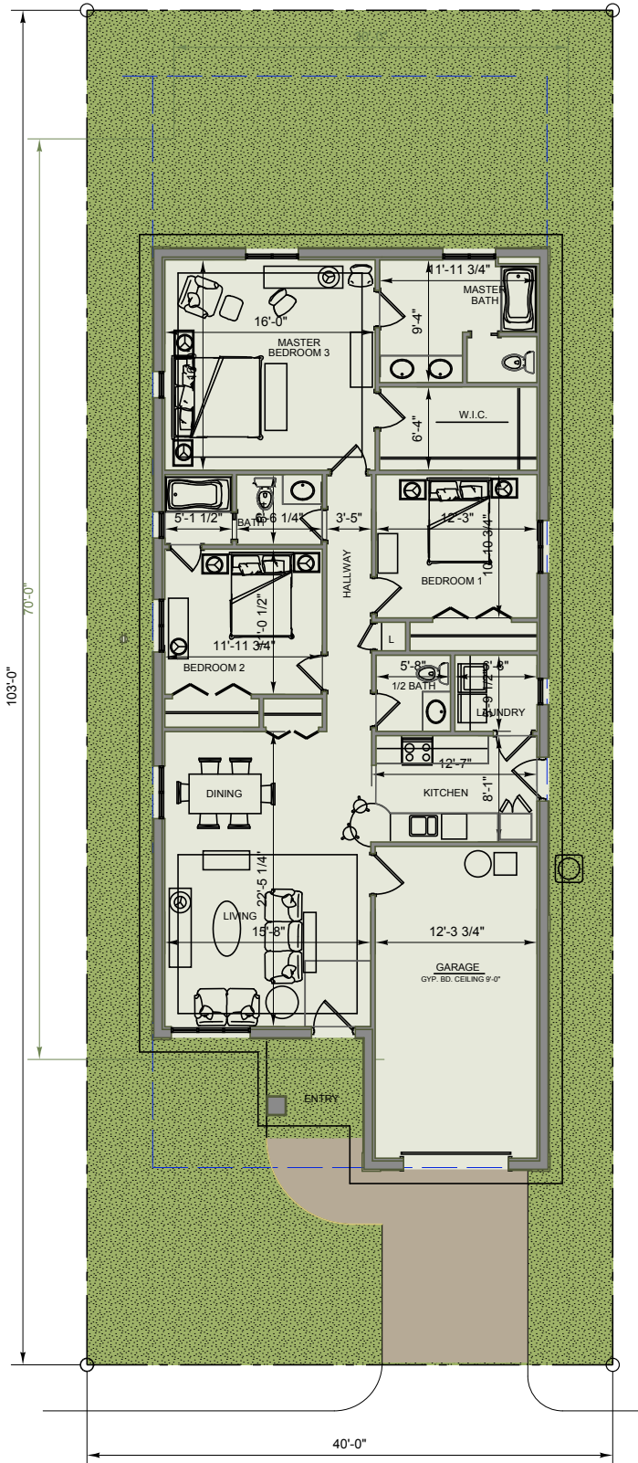
FLOOR PLAN
